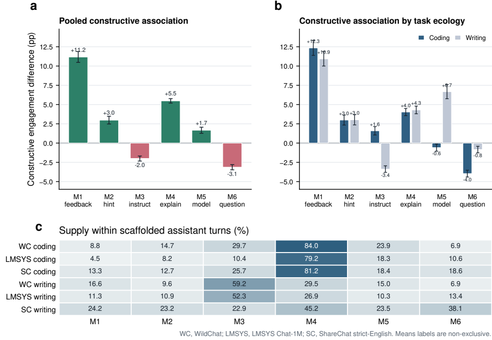
Fig. 4 Support form and support supply differentiate scaffolded interaction. a , Pooled constructive-engagement differences associated with each support form among scaffolded conversations across the six public-chat task settings. b , The same support-form contrasts stratified by coding-versus writing-oriented task ecology. c , Percentage of scaffolded assistant turns containing each support form by task setting. Bars compare scaffolded conversations containing a support form with scaffolded conversations without that form; error bars show 95% confidence intervals. Support-form labels correspond to M1–M6 and are not mutually exclusive, so rows do not sum to 100%.
