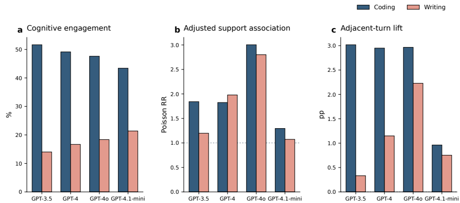
Fig. D9 WildChat model-family summary. WildChat model snapshots are grouped into coarse model families to summarize cognitive engagement prevalence, adjusted support associations and adjacent-turn constructive lift.
