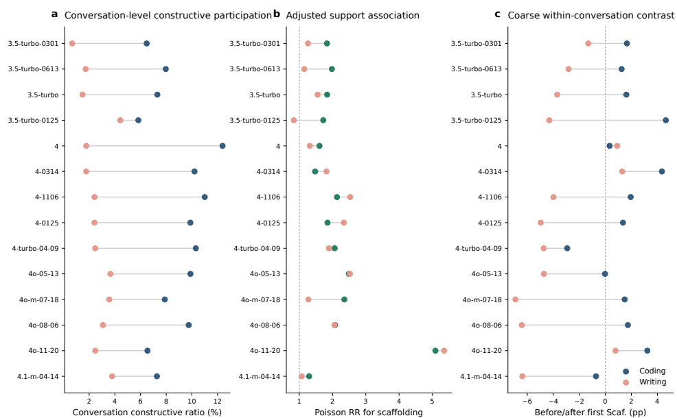
Fig. D7 Conversation-level support associations by WildChat model snapshot. The figure reports constructive participation, adjusted support associations and coarse before–after summaries around the first scaffolded assistant turn by user-facing WildChat model snapshot.
