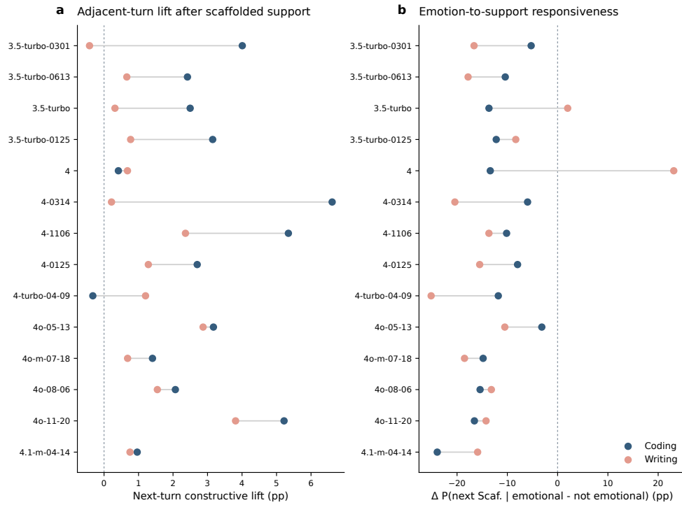
Fig. D8 Adjacent-turn summaries by WildChat model snapshot. The figure reports adjacent-turn constructive lifts and emotion-to-support responsiveness by user-facing WildChat model snapshot.
