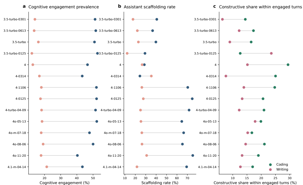
Fig. D5 WildChat model-snapshot prevalence profiles. The figure reports cognitive engagement, constructive engagement and scaffolded-support prevalence by user-facing WildChat model snapshot and task setting.
