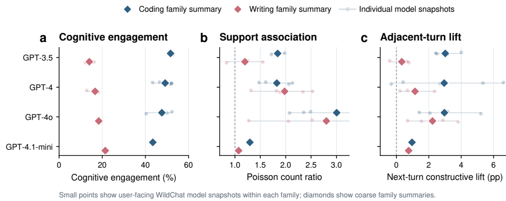
Fig. D2 WildChat model-family robustness preserves the main directional patterns. User-facing WildChat model snapshots are grouped into coarse model families. Diamonds show family-level summaries; small pale points show individual model snapshots within each family. a , Cognitive engagement prevalence. b , Adjusted scaffolded-support association, reported as Poisson count ratios. c , Adjacent-turn constructive lift after scaffolded versus reference assistant turns. The figure is descriptive because WildChat model labels are observational and may reflect time, user mix, task mix and logging context.
