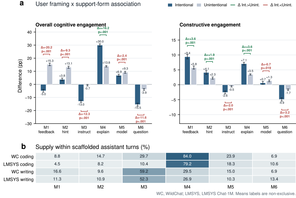
Fig. 4 Support form, user framing and support supply differentiate scaffolded interaction. a , Engagement differences associated with each support form among scaffolded WildChat and LMSYS conversations, stratified by intentional versus unintentional learning orientation. Bars compare scaffolded conversations containing a support form with scaffolded conversations without that form; error bars show 95% confidence intervals, and brackets compare intentional and unintentional contrasts. b , Percentage of scaffolded assistant turns containing each support form by task setting. Support-form labels correspond to M1–M6 and are not mutually exclusive, so rows do not sum to 100%.
