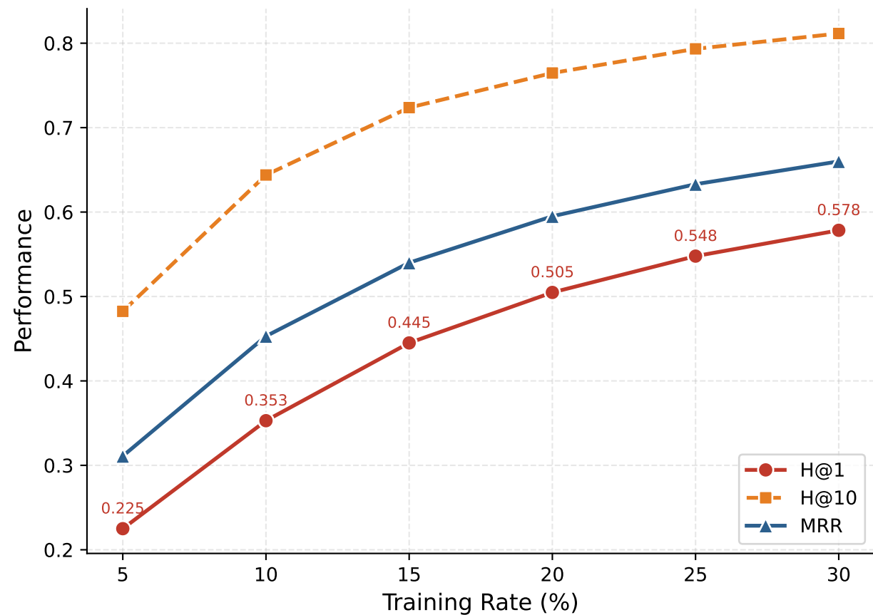
FB15K-DB15K
