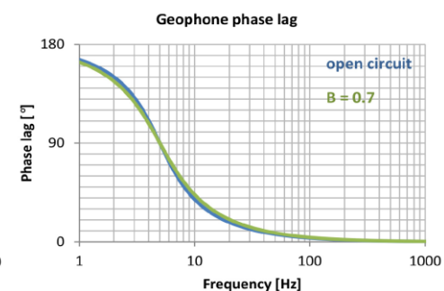
5Hz High Sensitivity Geophone Response Curve and Phase Lag
