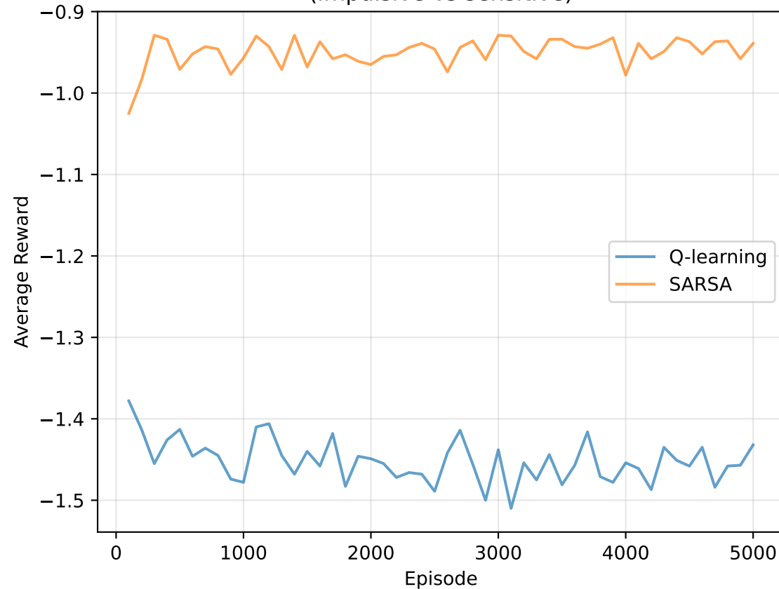
C1: Q-learning vs SARSA (impulsive vs sensitive)
