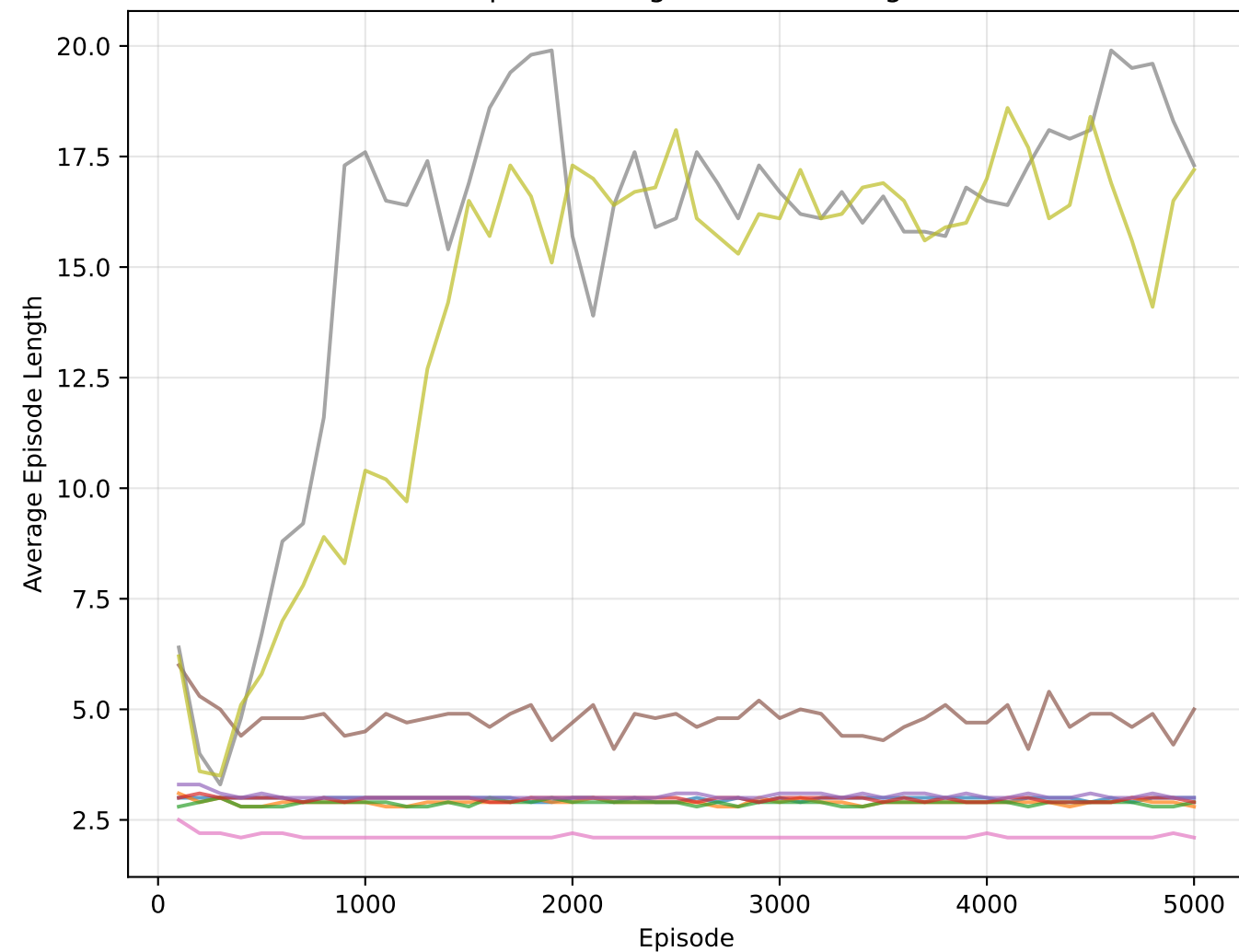
Episode Length Over Training
