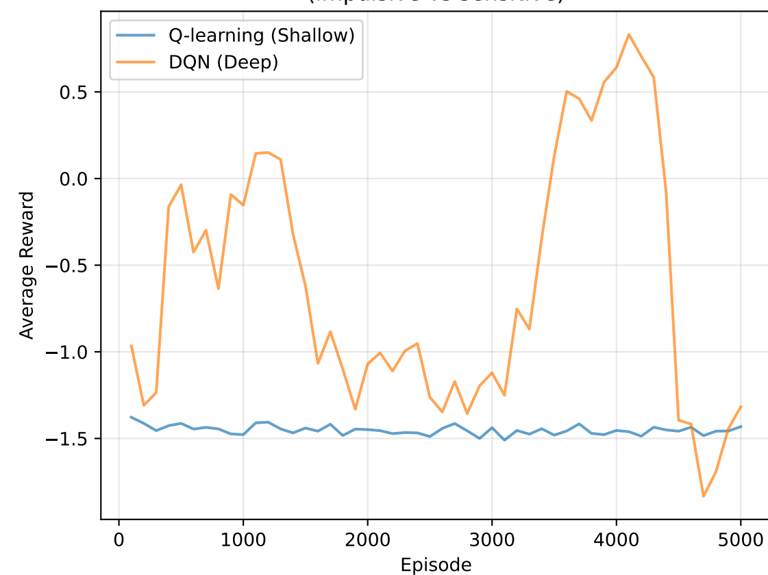
C3: Shallow vs Deep RL (impulsive vs sensitive)
