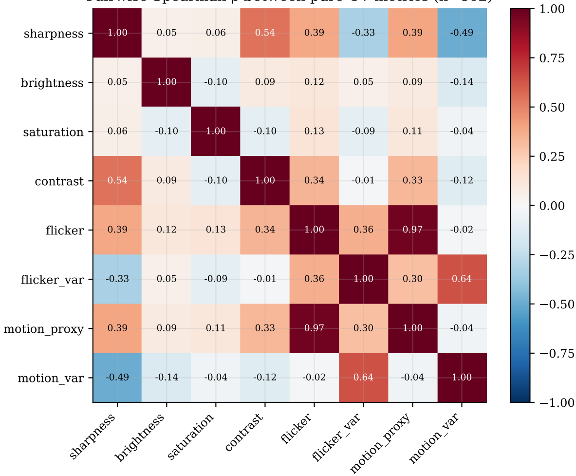
Pairwise Spearman \rho between pure-CV metrics (n=862)
