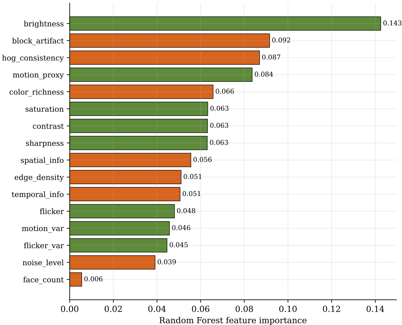
Feature importance — RF on combined 862 videos. Orange = new in v0.4.10.1; green = baseline.
