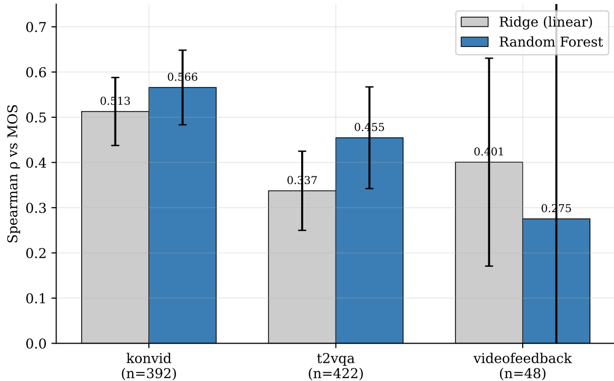
Per-dataset oracle (16 features, 5-fold CV) RF beats Ridge by +0.05 (KoNViD), +0.12 (T2VQA), -0.13 (VF, n too small)
