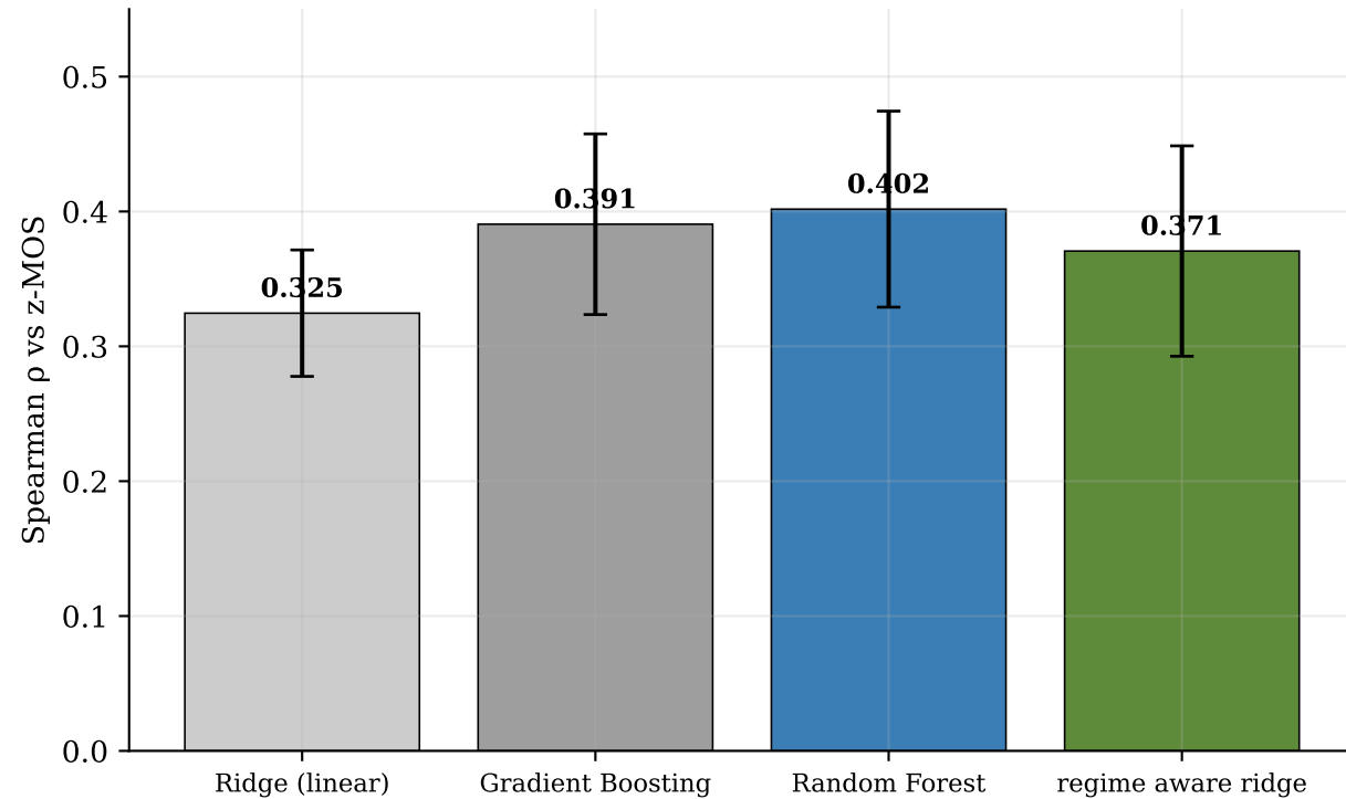
Combined n=862 — 5-fold stratified CV Random Forest beats linear Ridge by +0.077
