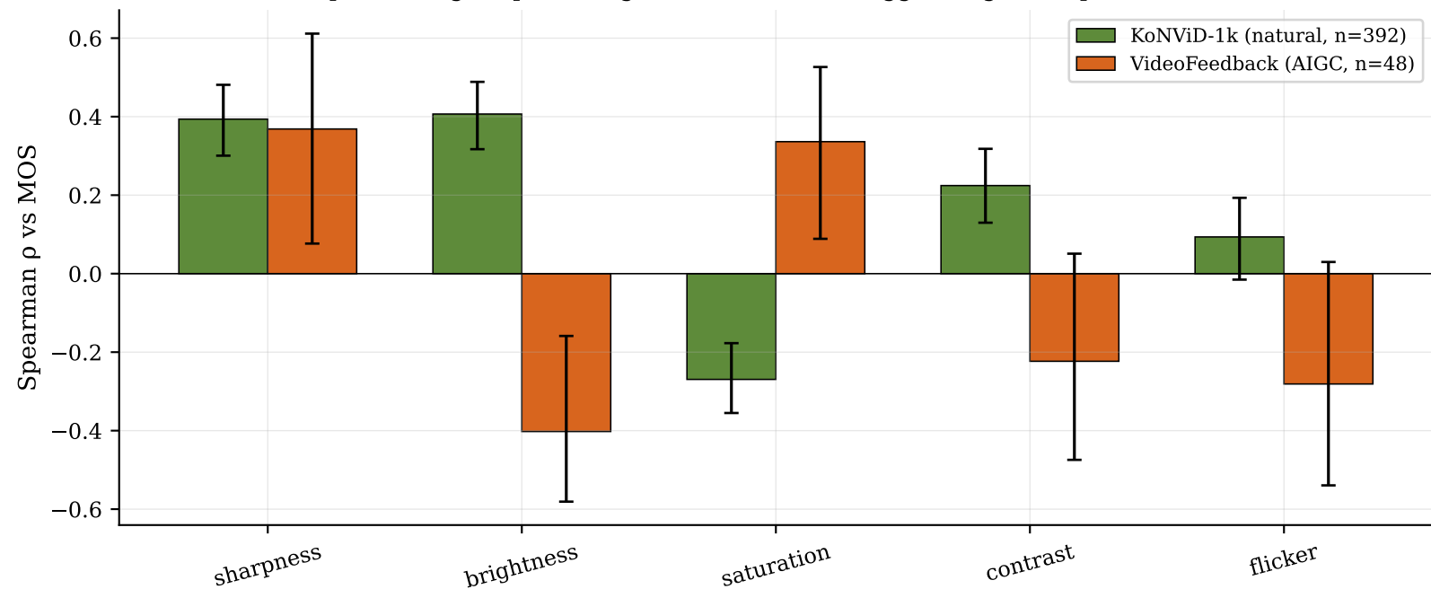
Natural-video vs AIGC: per-metric correlation with human MOS Bootstrap CI95. Sign-flips on brightness/saturation suggest regime-dependent calibration.
