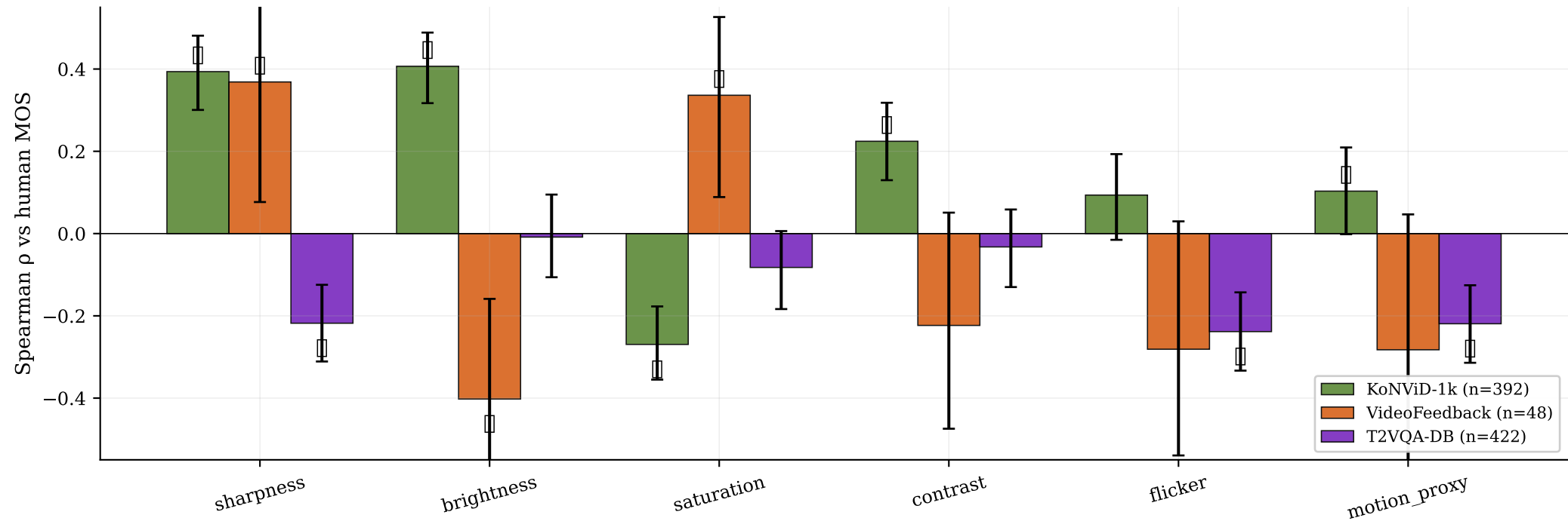
Pure-CV metrics across three regimes — natural video, small AIGC, large AIGC. □ = FDR-significant (Benjamini-Hochberg \alpha=0.05 ). Error bars = bootstrap CI95 (n_boot=2000).
