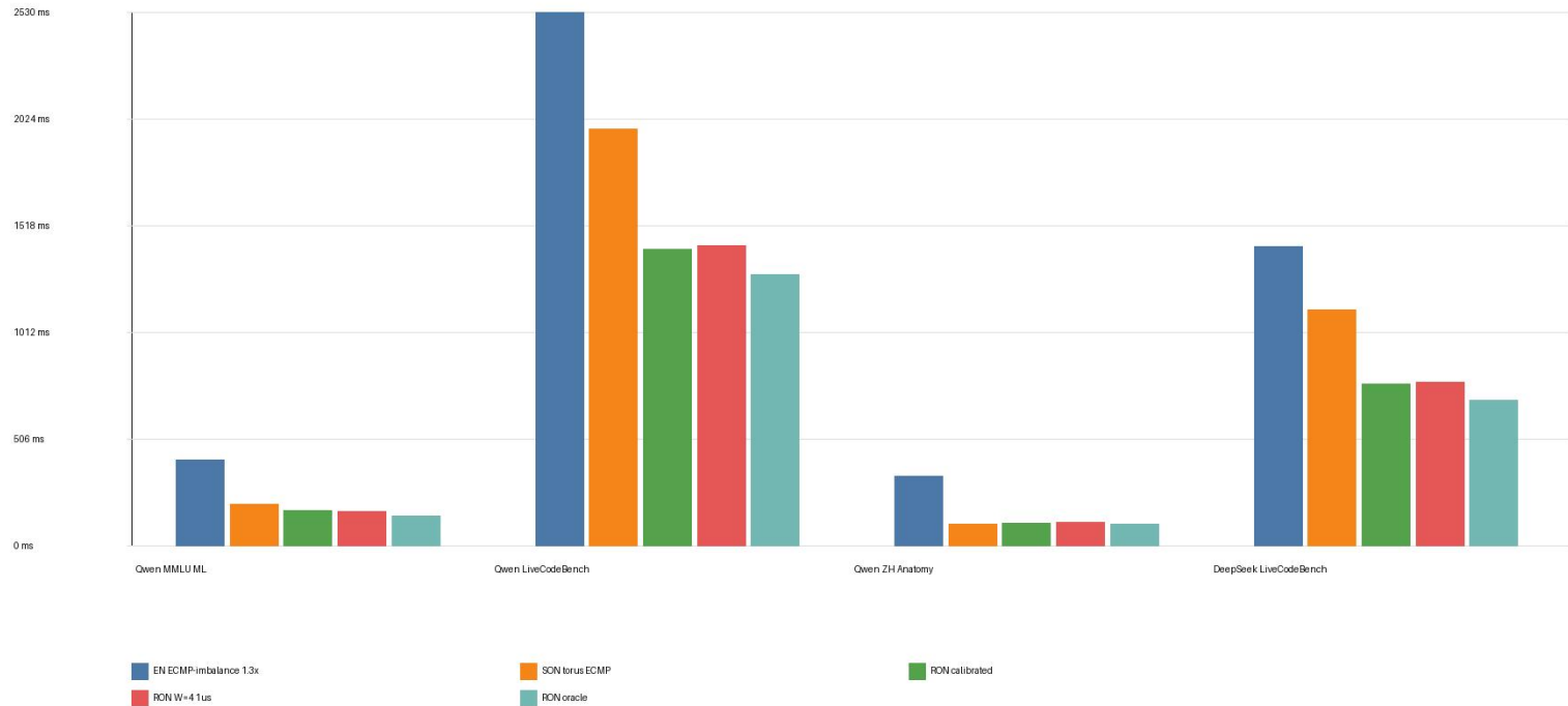
32-GPU MoE Prefill Communication Time
