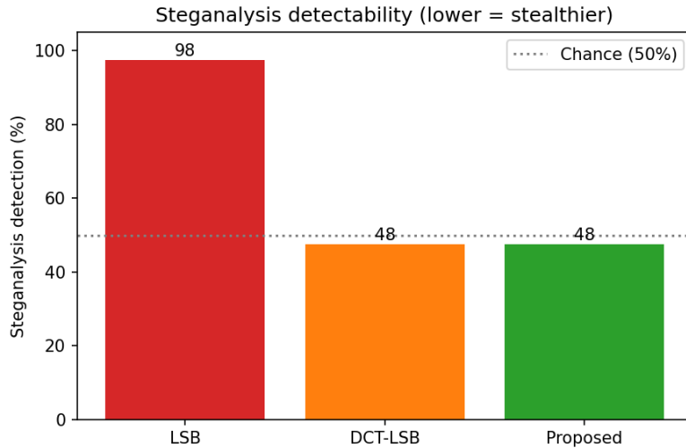
Figure 11: (Table 7) Measured steganalysis detection rates (lower is stealthier). LG-CISH sits at the chance line, far below LSB.
