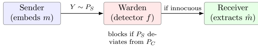
Figure 1: The prisoner’s problem. The transmitted object passes only if the warden’s detector cannot separate its law P_S from the natural-image law P_C . Security is a statement about distributions, not about pixels.
