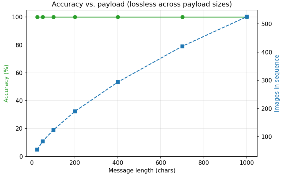
Figure 7: Reconstruction accuracy vs. payload length: 100% across all sizes while the image count grows linearly (matches Table 2).
