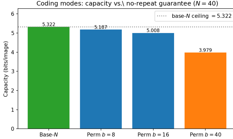
Figure 5: Capacity per image for base- N vs. permutation coding at several block sizes (matches Table 4). Smaller permutation blocks recover most of the base- N ceiling while guaranteeing no in-block image repeats.
