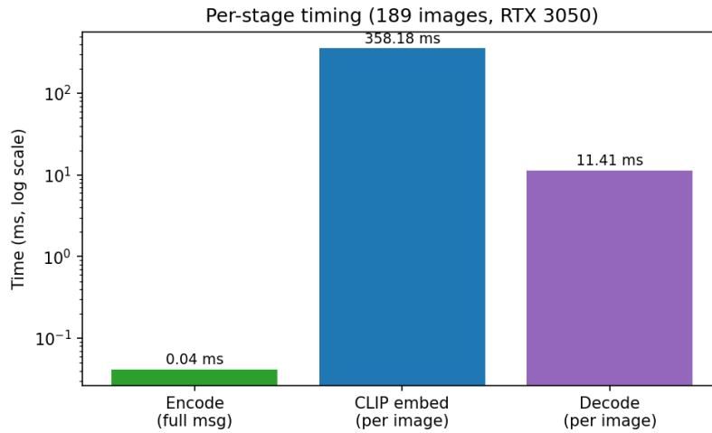
Figure 6: Per-stage timing on log scale (matches Table 5). Encoding is sub-millisecond; cost is dominated by CLIP embedding at decode.
