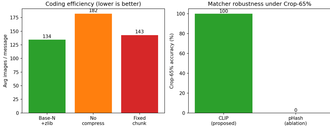
Figure 12: Left: base- N + zlib needs the fewest images. Right: under Crop-65% CLIP keeps 100% while pHash drops to 0% (matches Table 10).
