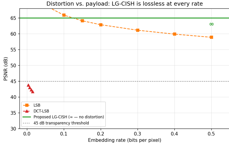
Figure 8: Capacity (bits/pixel) vs. distortion (PSNR). LG-CISH sits at infinite PSNR — no pixel is modified (matches Table 3).
