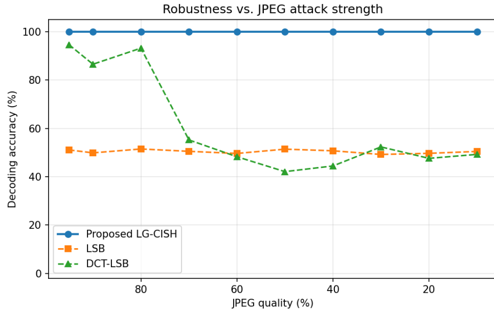
Figure 10: Decoding accuracy vs. JPEG quality: LG-CISH stays at 100% where pixel-domain LSB/DCT collapse.
