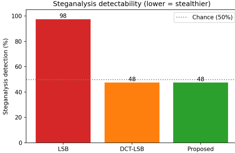
Figure 11: Measured steganalysis detection rates (lower is stealthier). LG-CISH sits at the chance line, far below LSB (matches Table 7).
