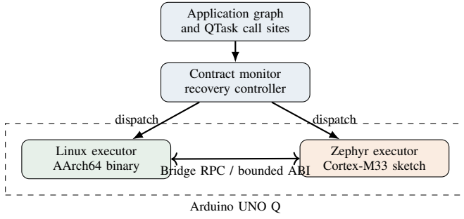
Fig. 1. QFabric architecture. The policy runs in Linux userspace; task code has a native implementation in each domain.
