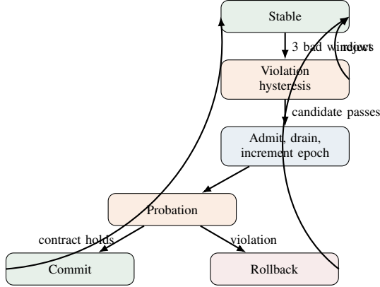
Fig. 2. Contract recovery. Prediction authorizes probation, not commitment.
