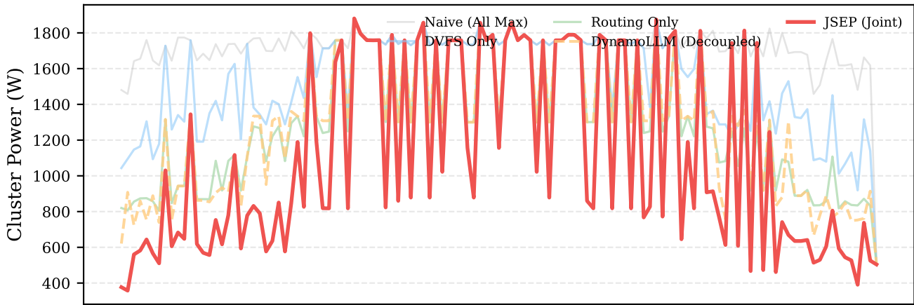
Power Over Time — Diurnal Trace (SLO = 500 ms)
