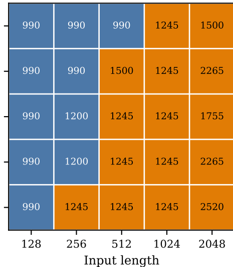
(c) P99 TTFT \leq 10000 ms
