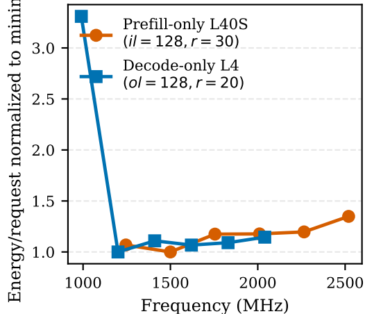
(b) Phase placement changes the efficient DVFS region
