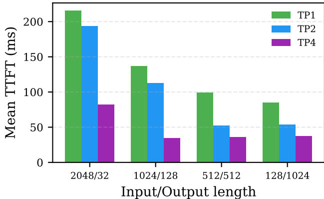
(a) Prefill latency (TTFT)
