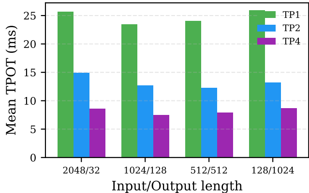
(b) Decode latency (TPOT)
