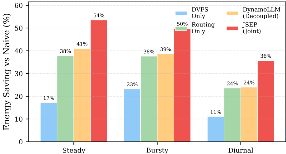
Energy Savings by Strategy (SLO = 500 ms)
