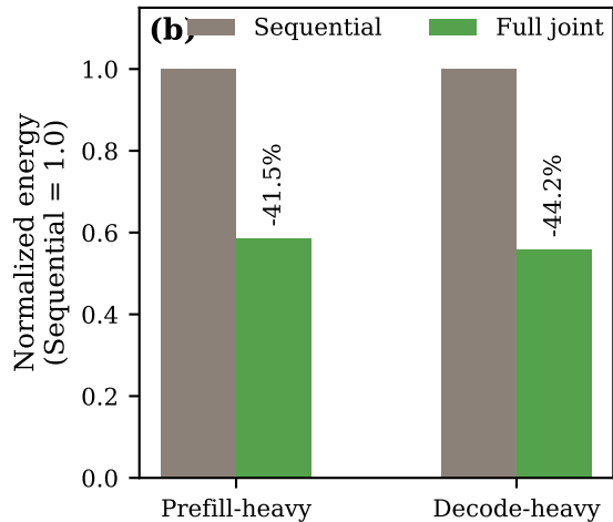
Sequential vs Full joint
