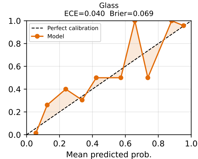
Stage 1 Reliability Diagrams (Calibration Curves) — Test Set CalibratedClassifierCV(method='sigmoid'); closer to diagonal = better calibrated
