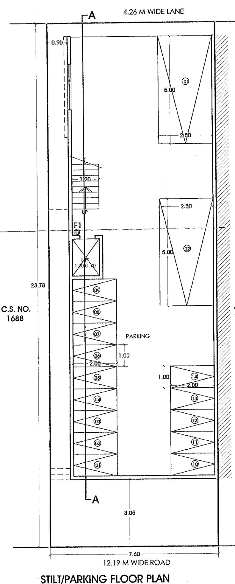
STILT/PARKING FLOOR PLAN
