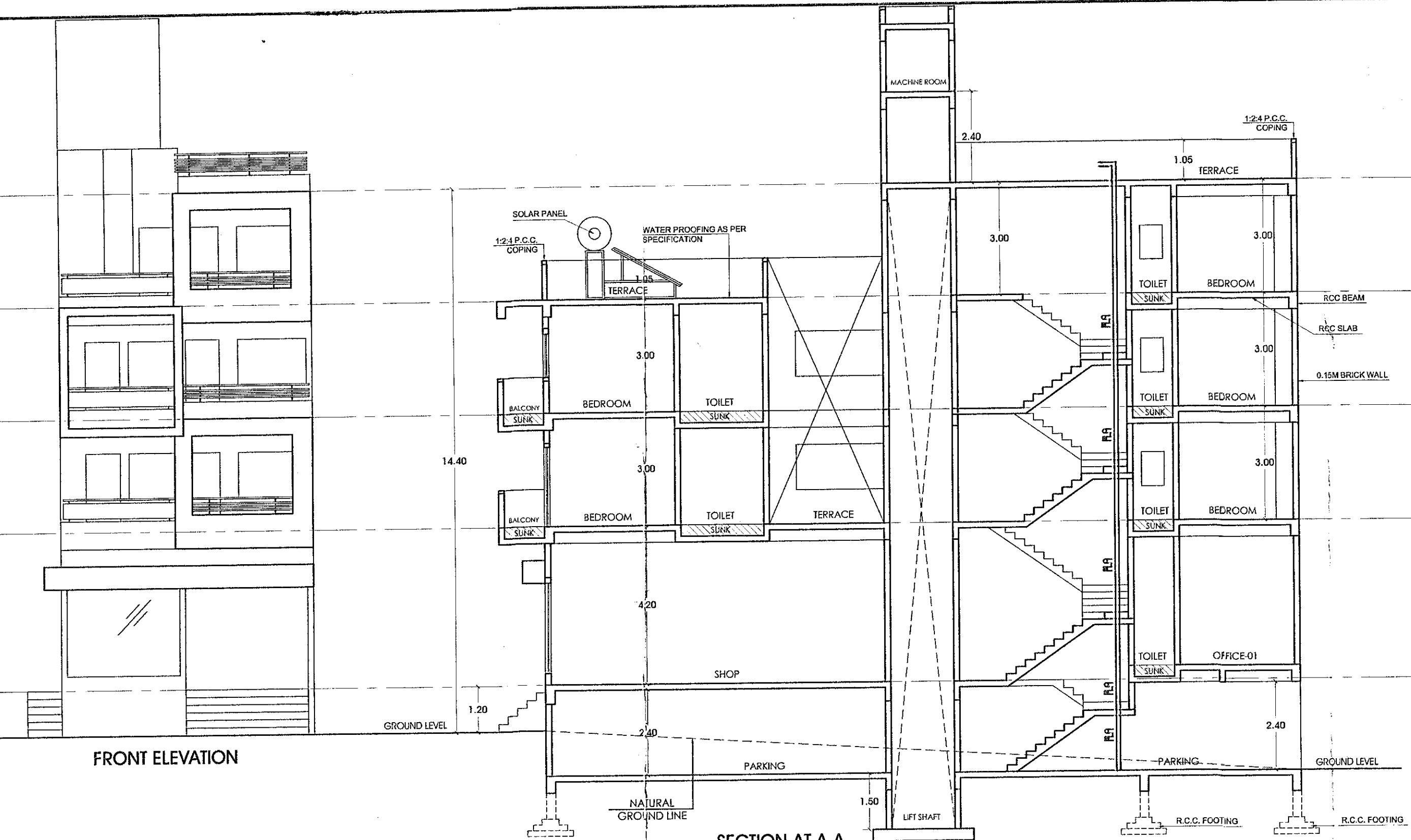
FRONT ELEVATION
