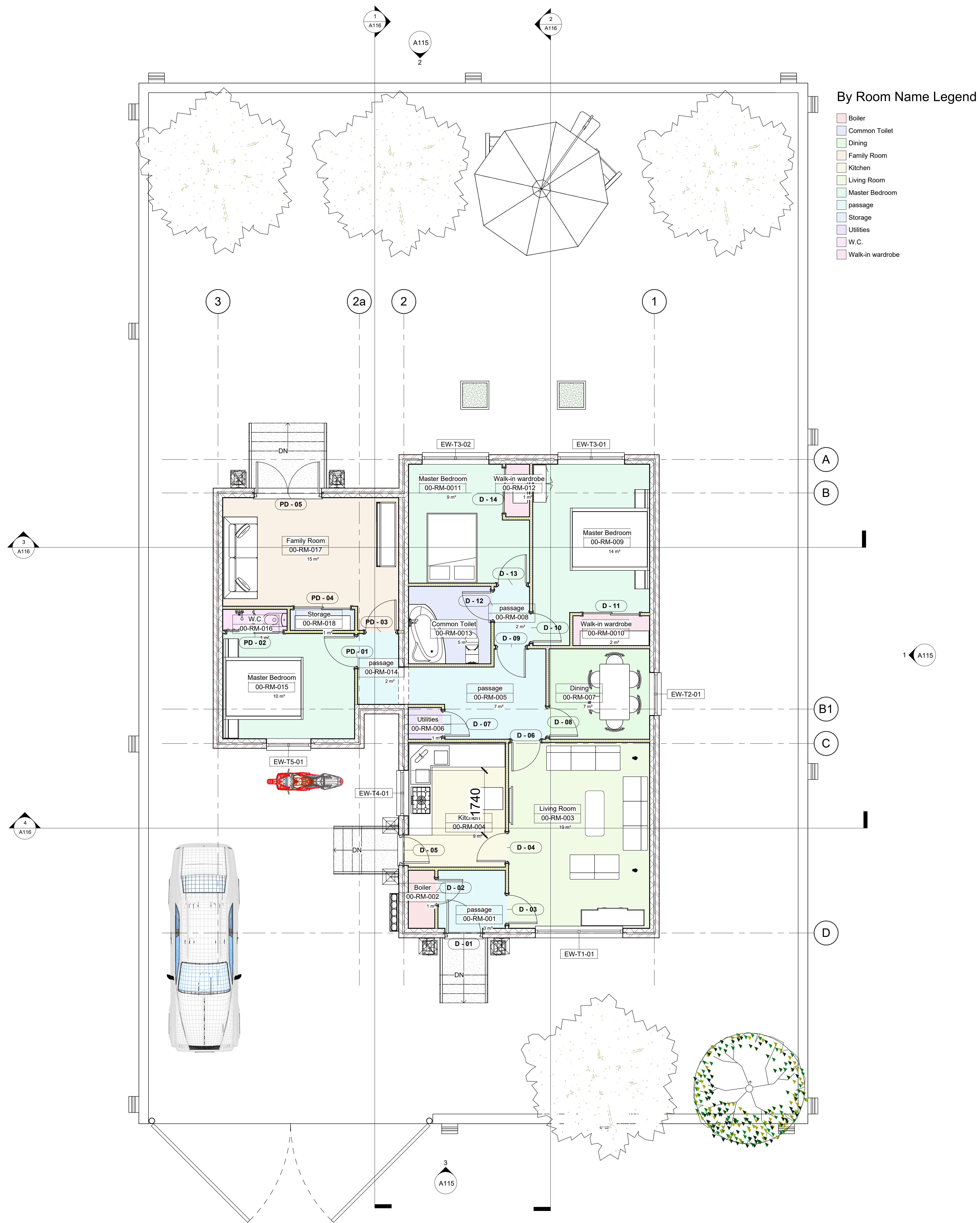
1 Level 00 Section Line 1 : 50
