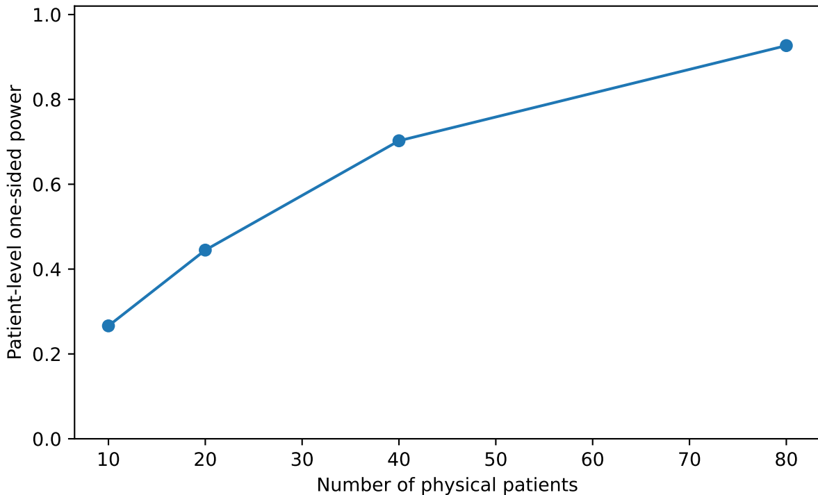
Independent patients, not cell rows, drive inferential power
