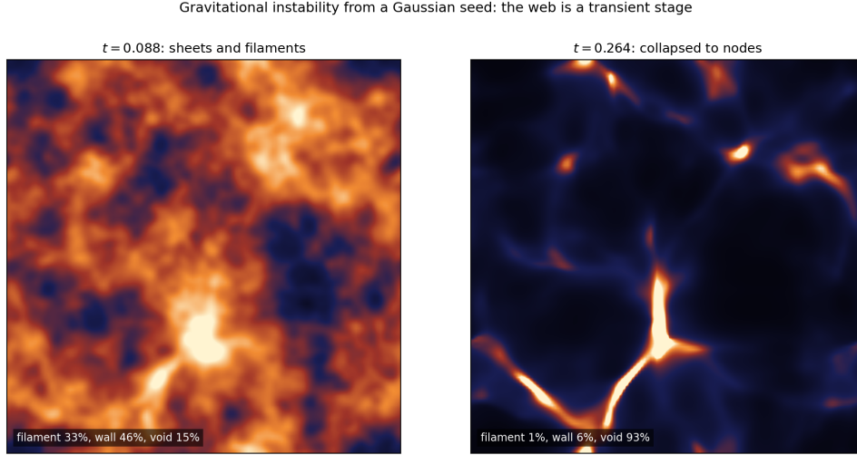
Figure 1: Gravitational instability of the contrast source (2) from a Gaussian seed ( 128^3 , thin slab; bright = overdense, dark = underdense). Left : sheet–filament stage, 33% filament and 46% wall by volume. Right : the same run later, collapsed to nodes, 1% filament and 93% void. The morphology is the classical Zel’dovich sequence [7], not particular to this model. Non-expanding box, so the web stage is transient.
