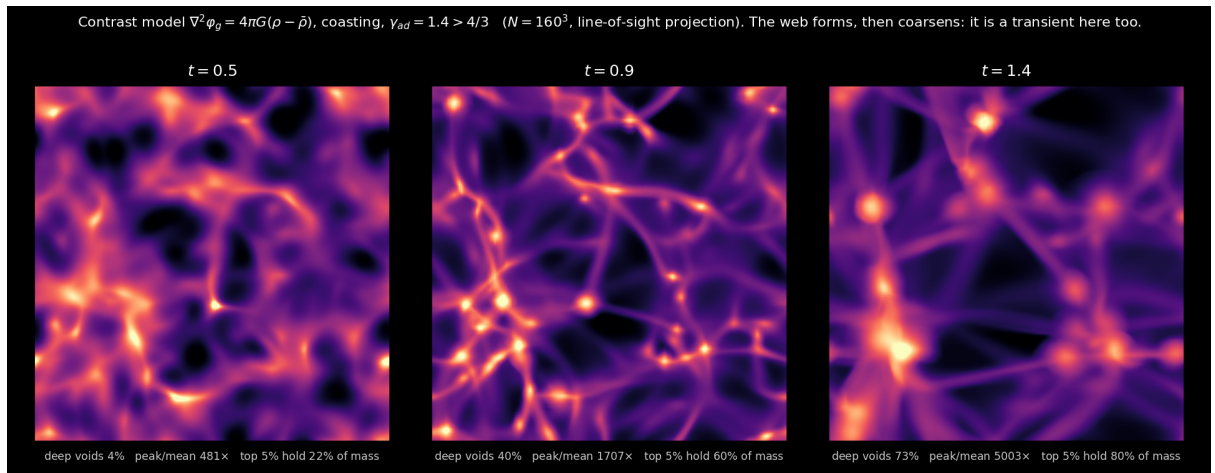
Figure 1: Gravitational instability of the contrast source (2) from a Gaussian seed, coasting background, \gamma_{\text{ad}} = 1.4 > 4/3 ( 160^3 , line-of-sight projection, logarithmic scale; bright = overdense). Filaments meeting at nodes with deep voids between, then coarsening. Total mass is conserved to 10^{-5} . The volume statistics drift by a few percent per refinement and the peak density not at all convergently (see text), so the morphology is indicative and the peak values are upper bounds set by the mesh. The morphology is the classical Zel’dovich sequence [8] and is not particular to this model; it illustrates the dynamics and is not offered as evidence for the cosmology.
