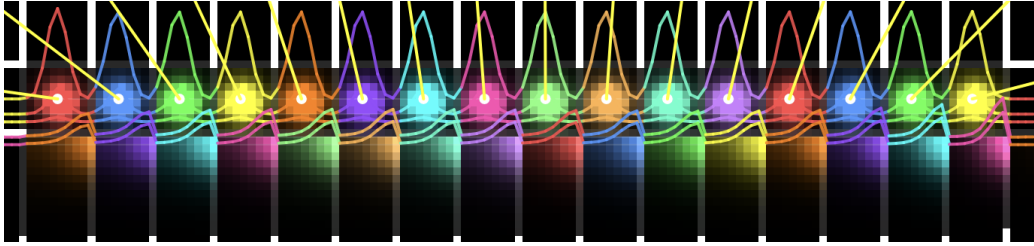
Figure 12.1: The cable, relaxed. Sixteen sites along the axis, each with a kernel of charge +3 , a core domain of two electrons confined within 2.4 a_0 , and one valence electron outside it. Colour distinguishes domains; white verticals mark the free boundaries between neighbouring carriers, the coloured curves are density profiles along the axis, and the yellow segments are net forces on the kernels. Every boundary shown is an unknown of the minimisation.
