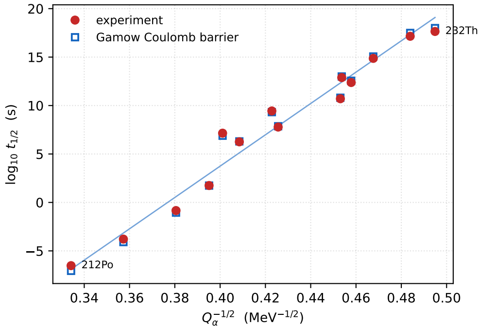
Geiger--Nuttall: one Coulomb barrier, 25 decades
