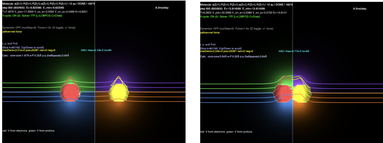
Figure 2: Fusion of two deuterons into the alpha, D + D \rightarrow {}^4\text{He} , computed directly. Each deuteron is built as a central electron core with its two protons split into halvespaces; the two deuterons are placed with their cores at separation 2R and relaxed at decreasing R . Left : the approach — the two deuterons still well separated. Right : the merged state — the two electron cores have joined into the central -2 glue (red/yellow) and the four protons into the quartal outer shell (blue/green): the dual-confined 2e + 4p alpha. The binding deepens monotonically as the cores approach — in the fully relaxed (adiabatic) coordinate the electron clouds screen the proton–proton repulsion at every separation, so the path into the alpha is downhill, the released energy being the fusion energy. Lower curves in each panel: the potential generated by the electrons (red) and by the protons (green).
