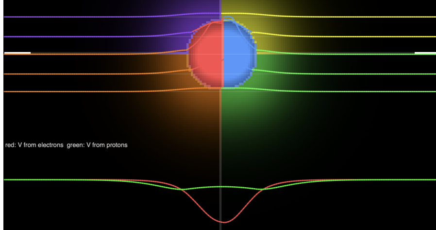
Figure 1: Dual confinement in the alpha ( 2e + 4p ), shown through the two Coulomb potentials. The potential generated by the electrons (red) is a deep central well that attracts the protons inward; the potential generated by the protons (green) attracts the electrons outward toward the surrounding protons, depleting the core. Each species is held in place by the other’s potential — by Coulomb attraction alone, with no external or strong-force confinement.
