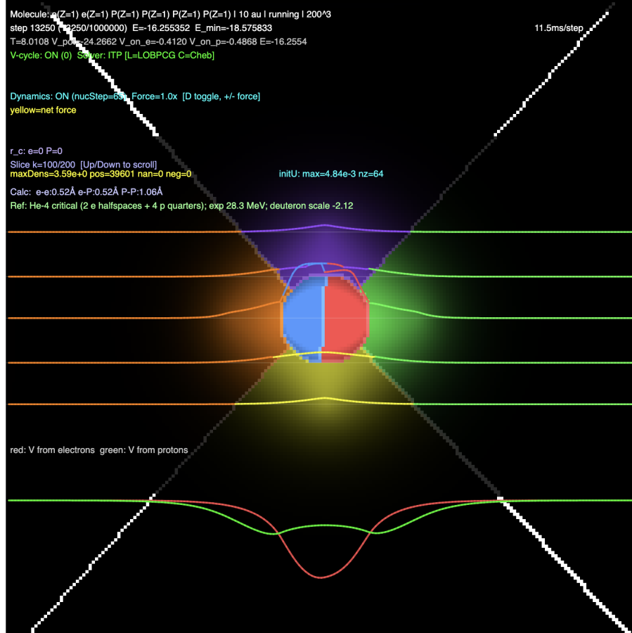
Figure 1: Dual confinement in the alpha, the main He-4 configuration: the two electrons split into halfspaces (red/blue) and the four protons into quarter pieces . Red is the potential generated by the electrons — a deep central well that pulls the protons inward. Green is the potential generated by the protons; note that it is not flat inside the electron core. By the shell theorem a spherically symmetric proton shell would give a constant interior potential and exert no force on the electrons; but the four discrete protons are not spherically symmetric, leaving a residual interior field that pulls the electrons outward toward the protons, depleting the core, and so cages them. Each species is held only by the other's Coulomb potential. The split of the two electrons into halfspaces is what enables the binding: a spherically symmetric electron core does not bind.
