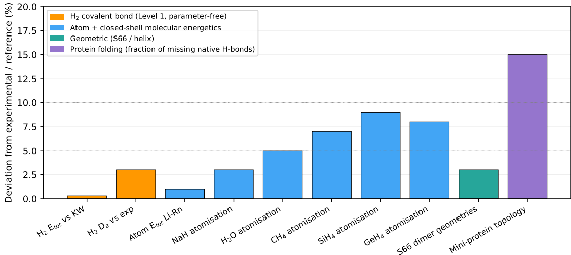
Figure 1: RealQM validation summary: deviation from experimental reference across regimes. Closed-shell molecular energetics (blue) sit at \sim 1 – 10\% across atoms and four periodic-table groups. The foundational H 2 covalent bond at parameter-free Level-1 (orange) matches Kolos–Wolniewicz to 0.3% on total energy and the experimental dissociation energy to 3%. Geometric matches against CCSD(T) and helix-geometry references (teal) are 3–5%. Protein-folding deviations (purple) are reported as the fraction of native H-bonds not formed. NaCl crystal melting (Section 4.13) is presented separately in the text: the simulation reproduces the qualitative phase-transition character (Lindemann ratio crossing, RDF peak collapse) but the absolute T_m is uncalibrated against experiment because the Brownian-dynamics time scale is not mapped to physical time — a calibration question, not a validation deviation, and it is therefore not plotted on this figure.
