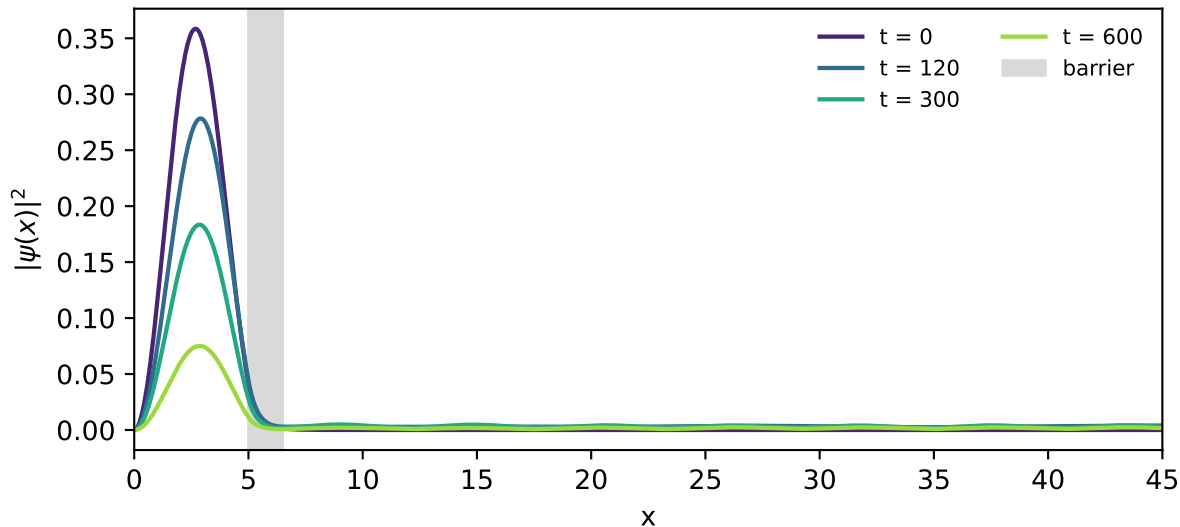
Full time-dependent RealQM: charge leaking through the barrier
