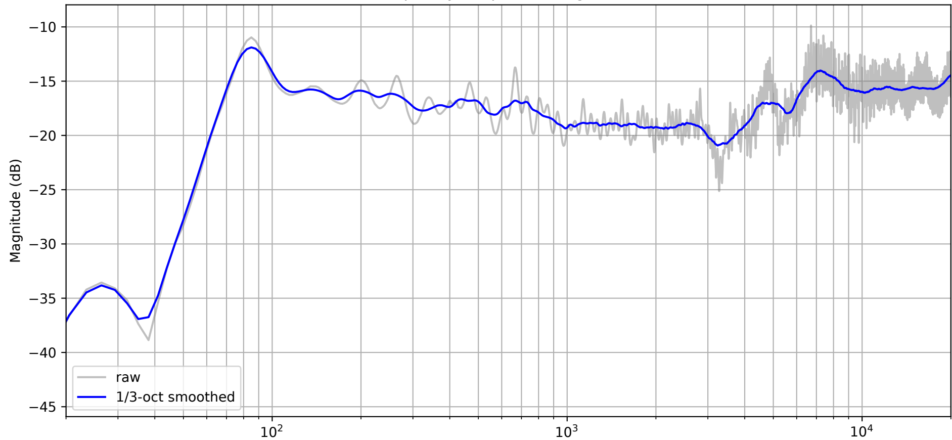
Frequency Response (Magnitude)
