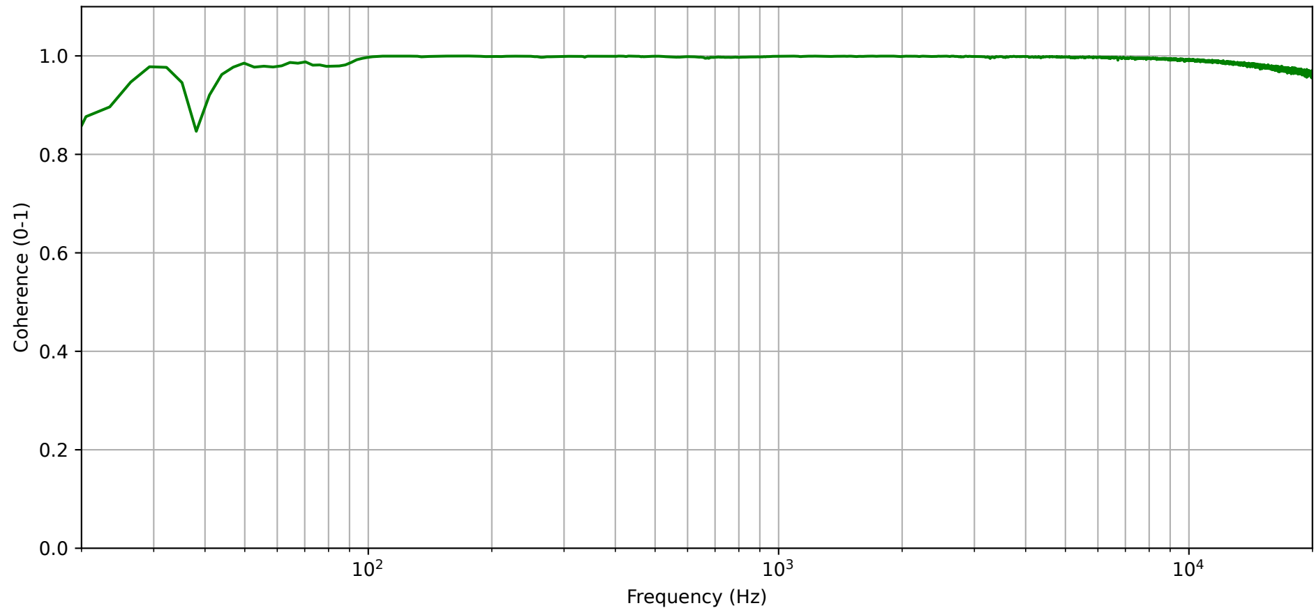
Coherence (Mean: 0.982)
