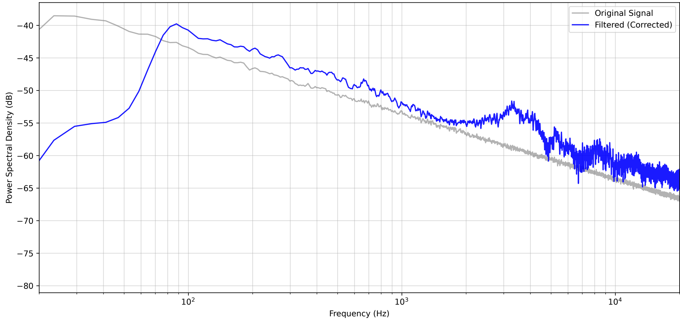
Spectrum Analysis: Before vs. After Correction
