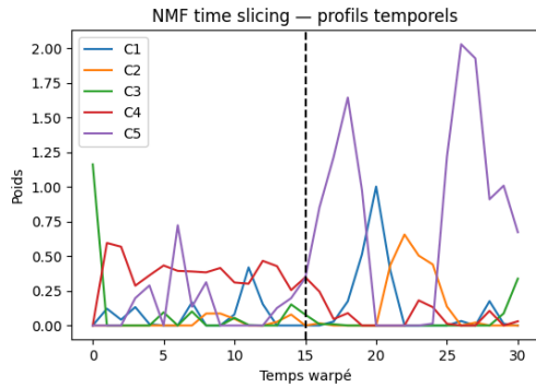
Fig. 12. Temporal components extracted by NMF after time slicing. Each curve corresponds to one component of W_{\text{time}} . The dashed vertical line indicates the puff-aligned bin.
