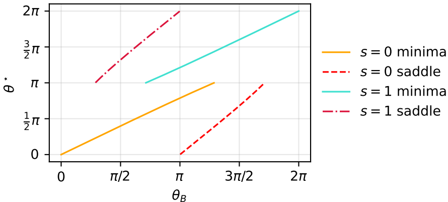
Boundary fixed points vs \theta_B for \kappa = 8
