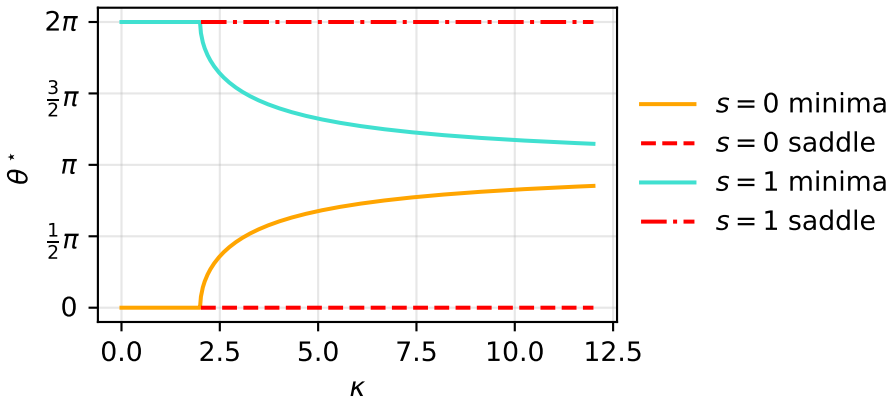
Boundary fixed points vs \kappa for \theta_B = \pi
