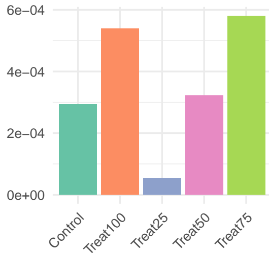
WS2
