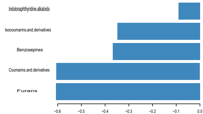
sPLS-DA: Component 1 Loadings
