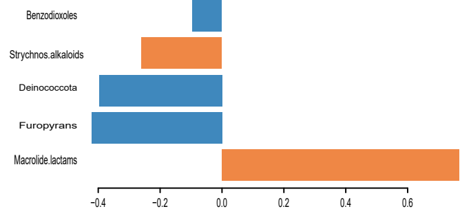
sPLS-DA: Component 2 Loadings
