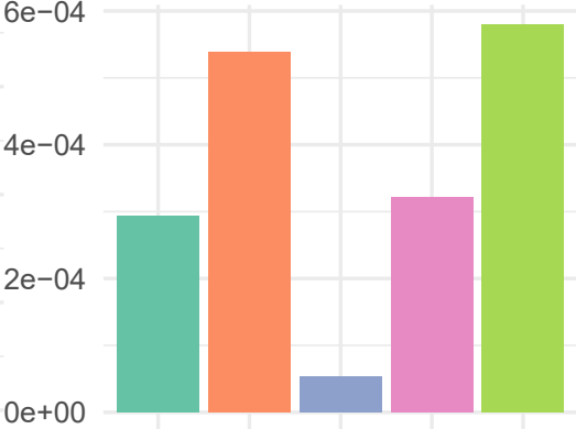
WS2
