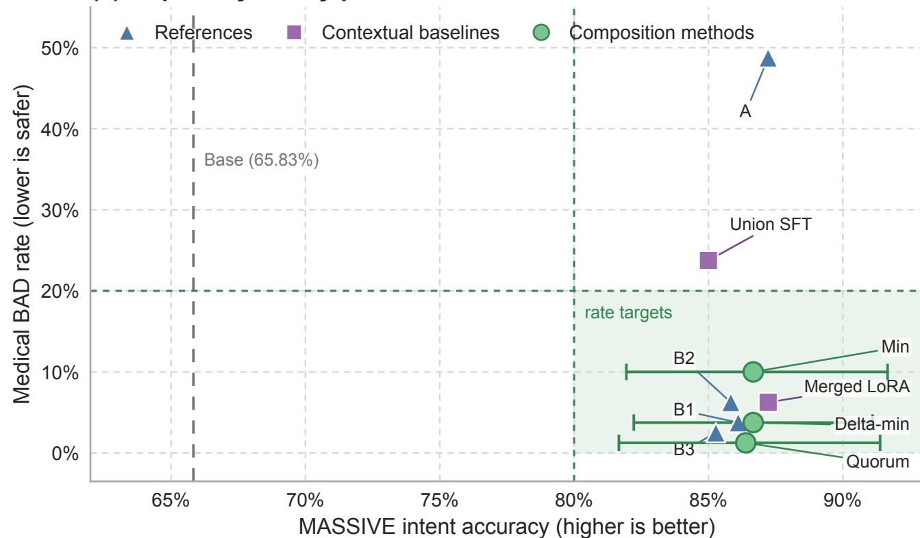
(a) Capability-safety plane
