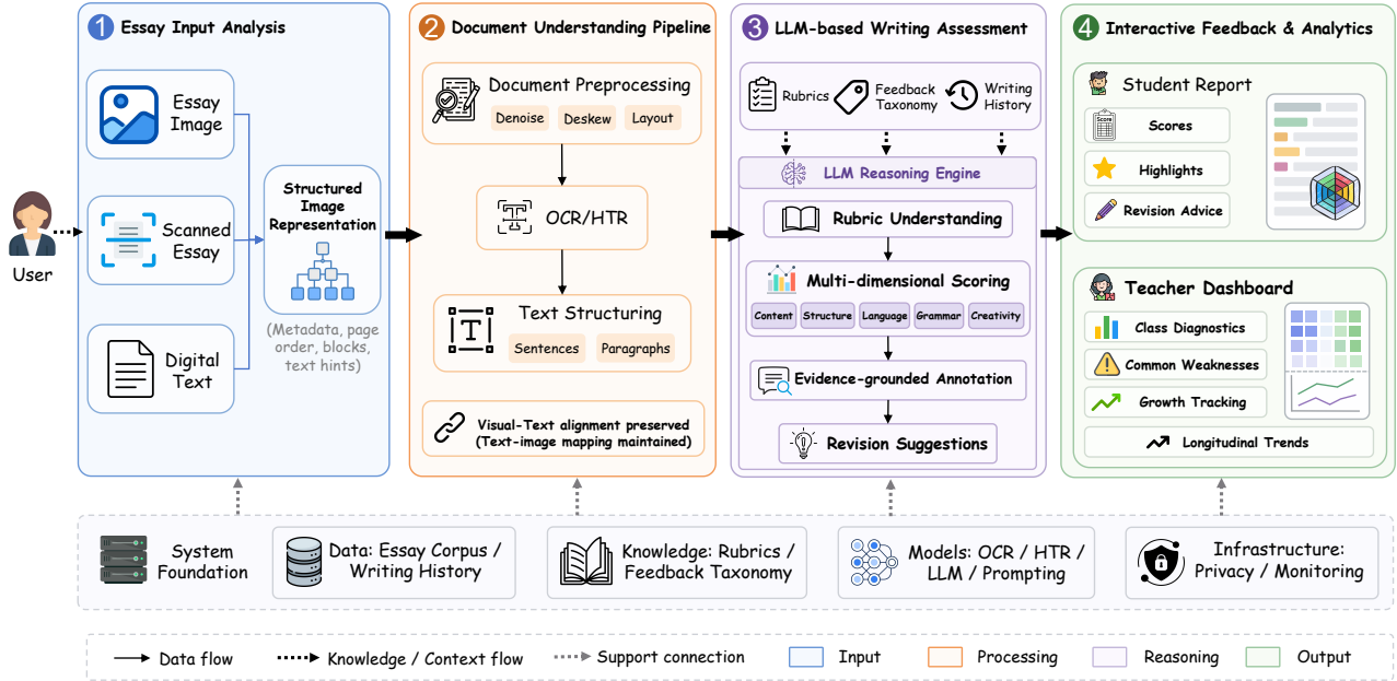
Figure 1: System architecture of QuickGrade.
