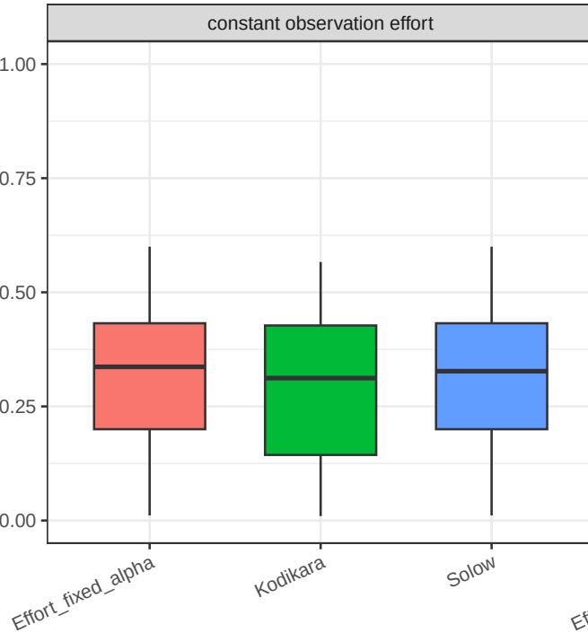
Posterior persistence probability in 2020
