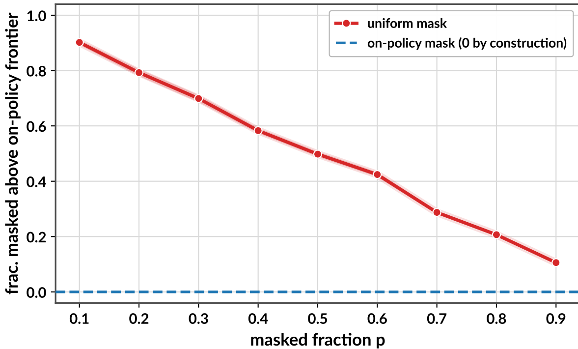
Fraction of masked tokens that are 'easy'
