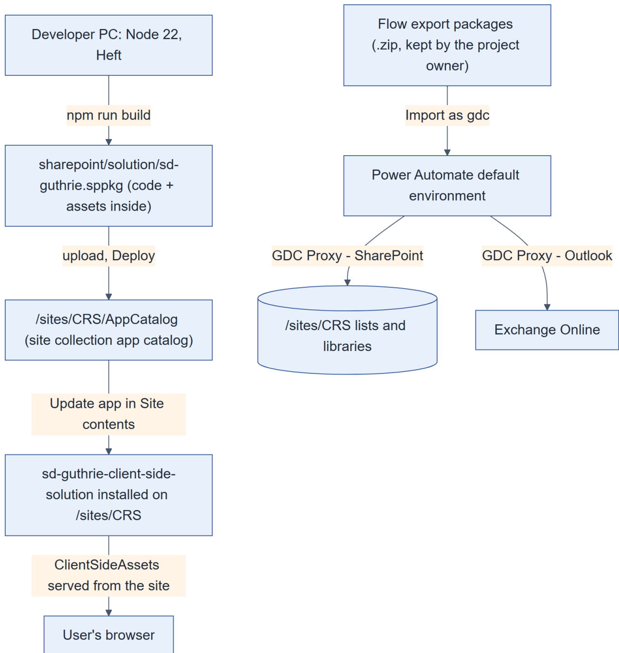
Figure 3. Deployment view
