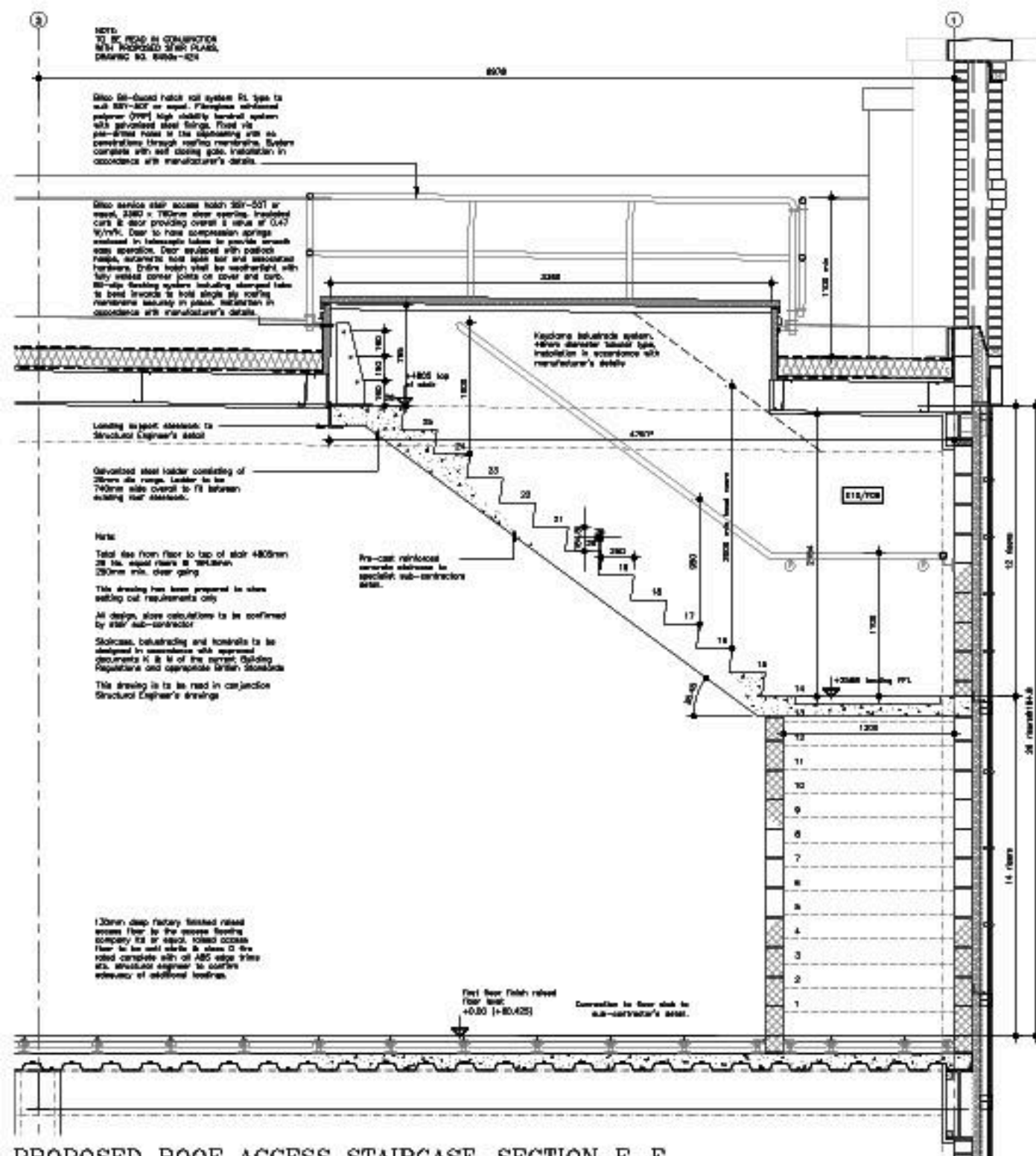
PROPOSED ROOF ACCESS STAIRCASE-SECTION E-E scale 1:20
