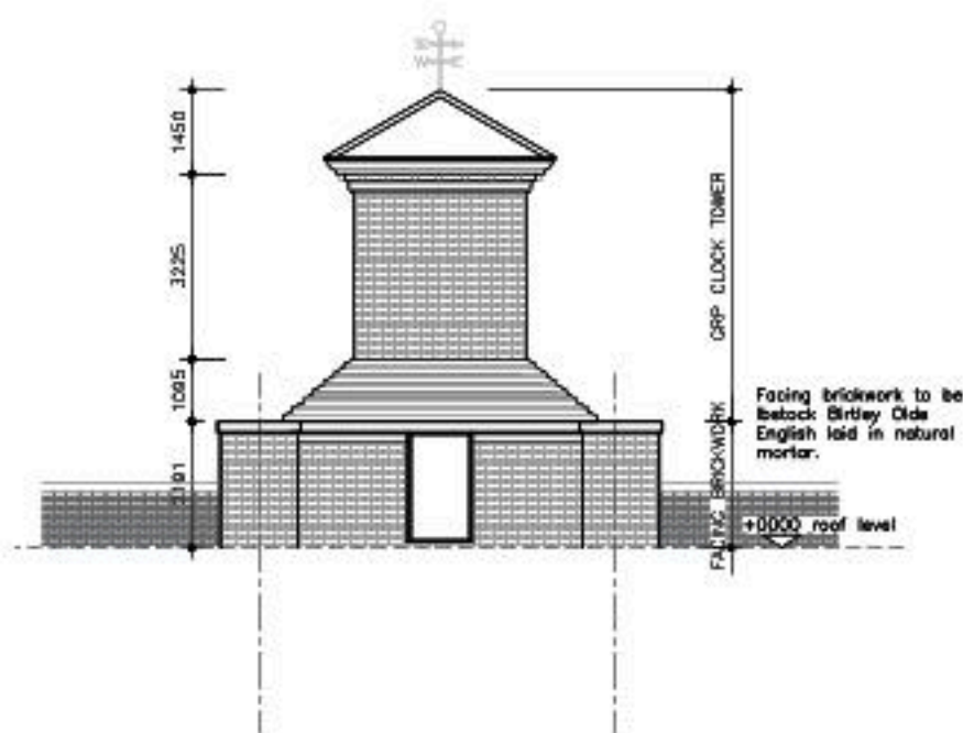
ELEVATION C
