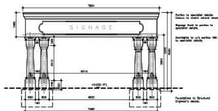
PROPOSED ELEVATION
