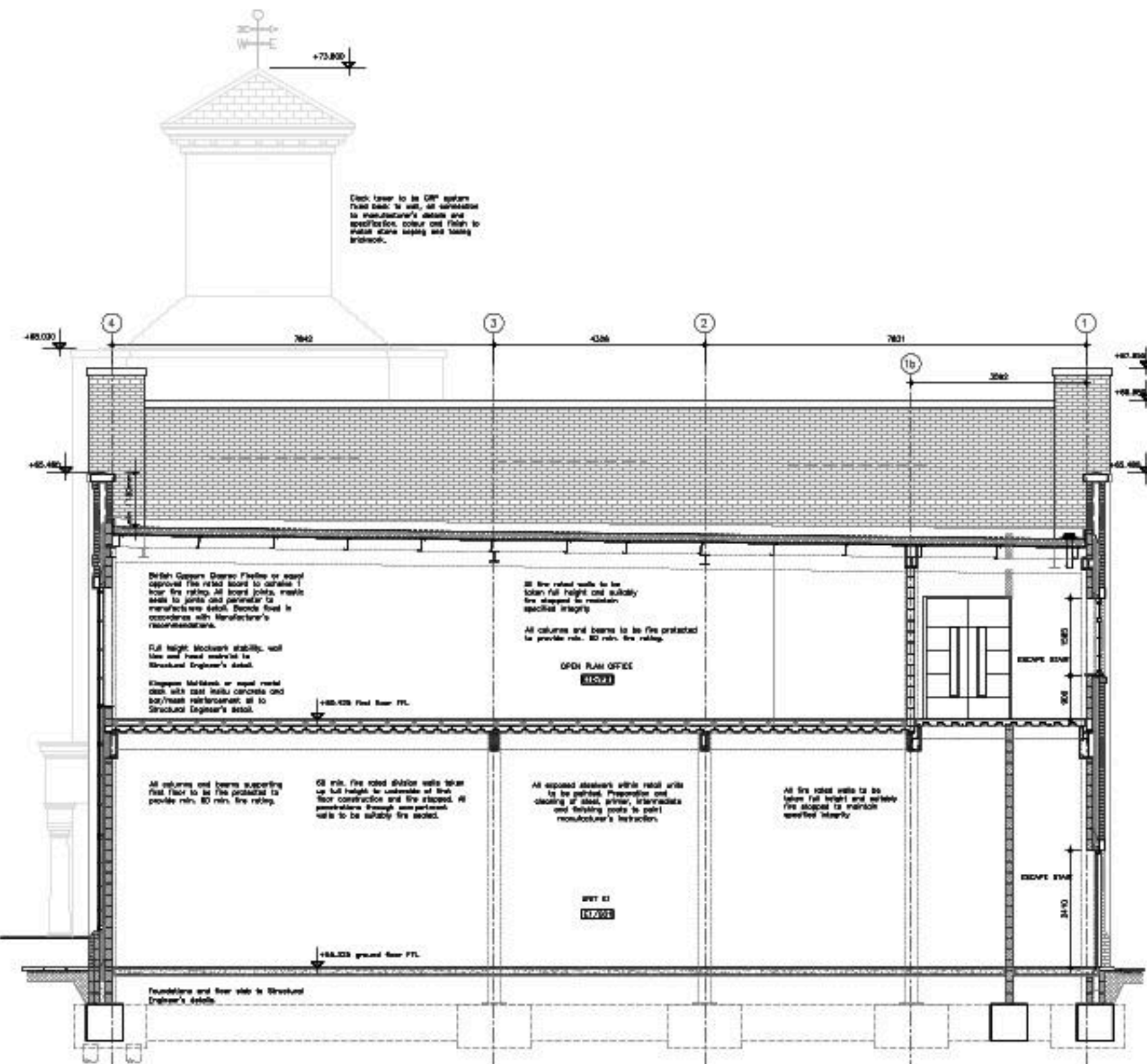
PROPOSED GENERAL ARRANGEMENT SECTION A-A BLOCK E Scale 1:50
