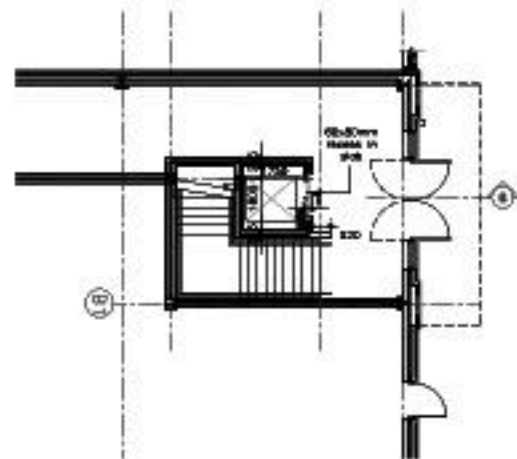
GROUND FLOOR PLAN OF LIFT PIT scale 1:100
