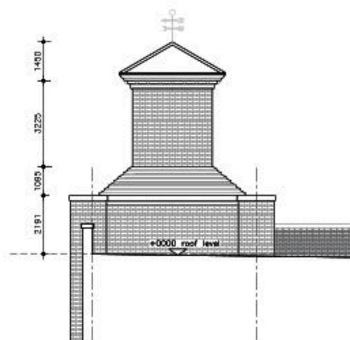
ELEVATION D
