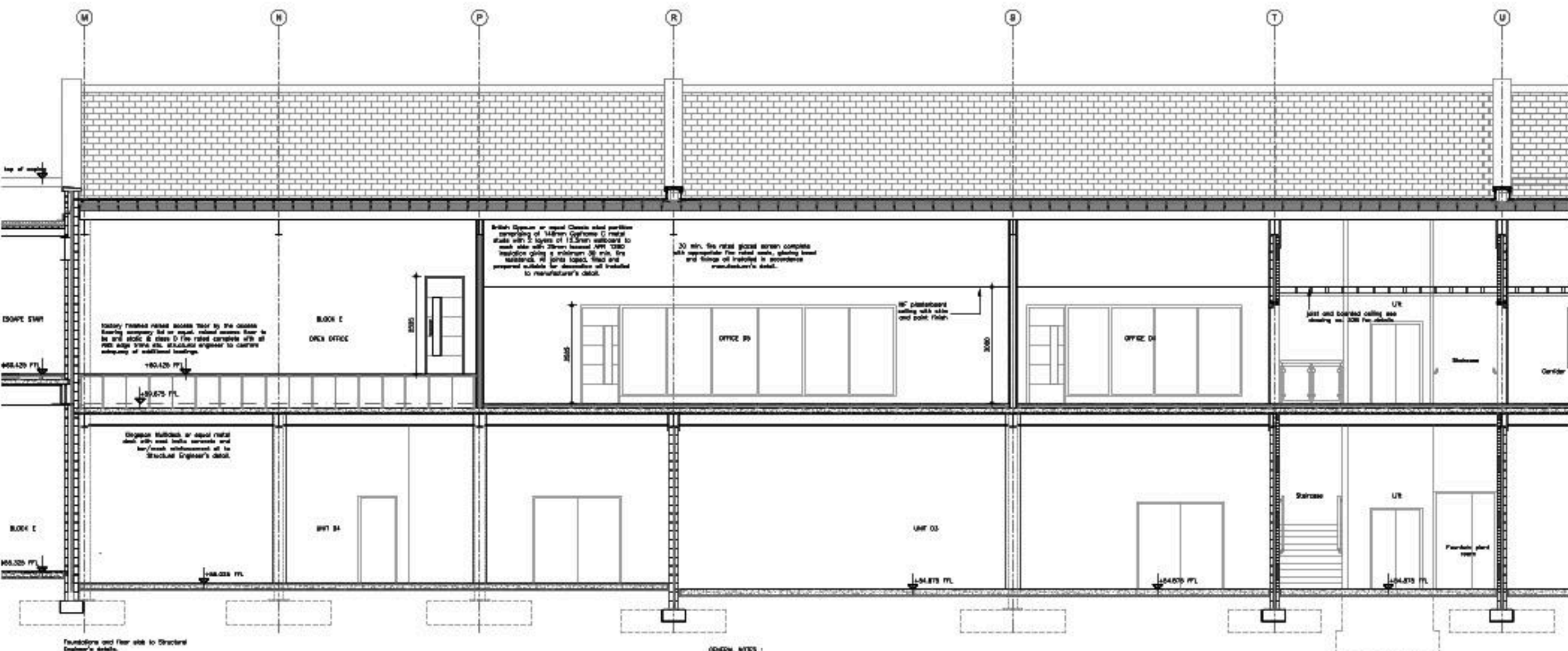
PROPOSED GENERAL ARRANGEMENT SECTION C-C, BLOCK D scale:1:50
