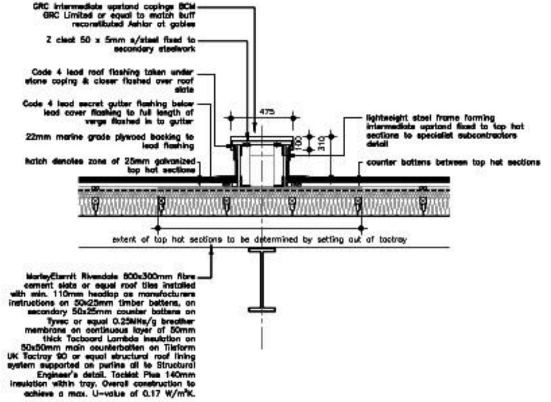
GRC INTERMEDIATE UPSTAND DETAIL BLOCK D scale 1:20
