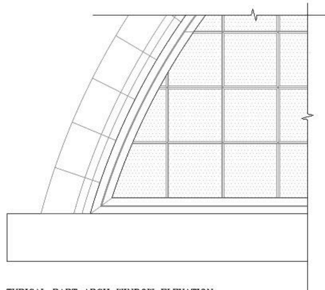
TYPICAL PART ARCH WINDOW ELEVATION
